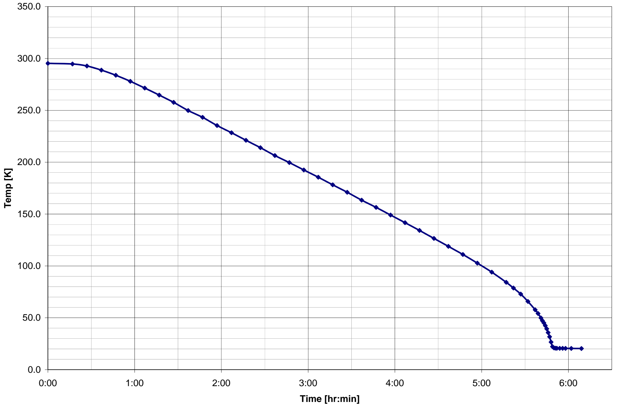
Scientia 2002 Cold Finger Cooling Curve (All components at room temperature at start)
